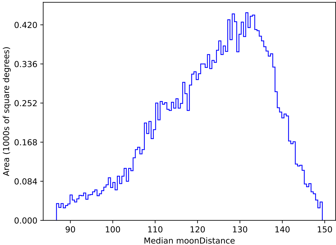
mw_roll_all_v3.3_10yrs All sky u band: Median moonDistance
