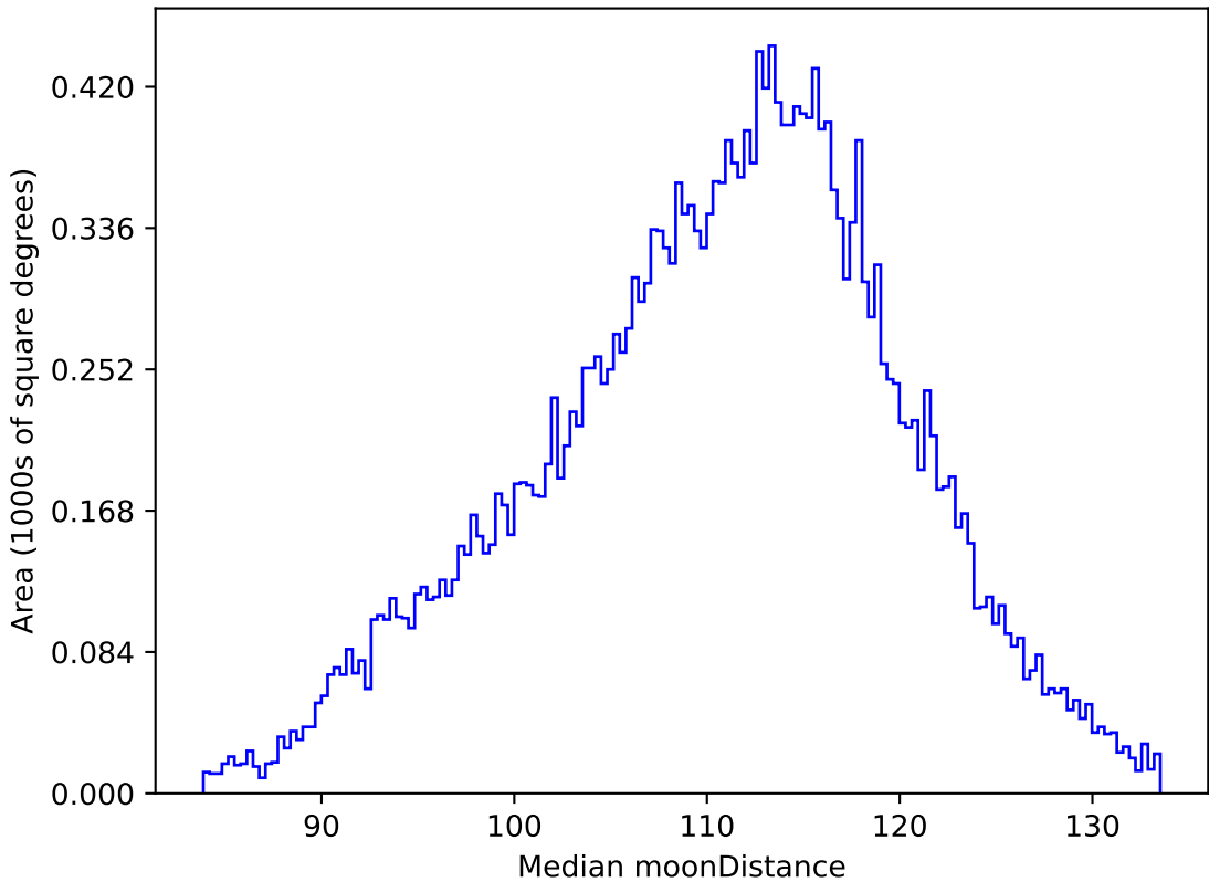
mw_roll_all_v3.3_10yrs All sky r band: Median moonDistance
