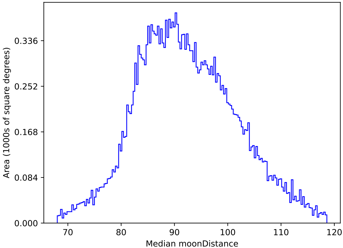
mw_roll_all_v3.3_10yrs All sky i band: Median moonDistance
