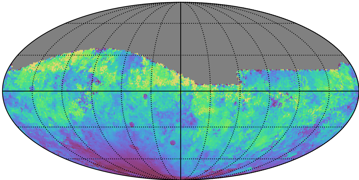
mw_roll_all_v3.3_10yrs All sky g band: Median moonDistance
