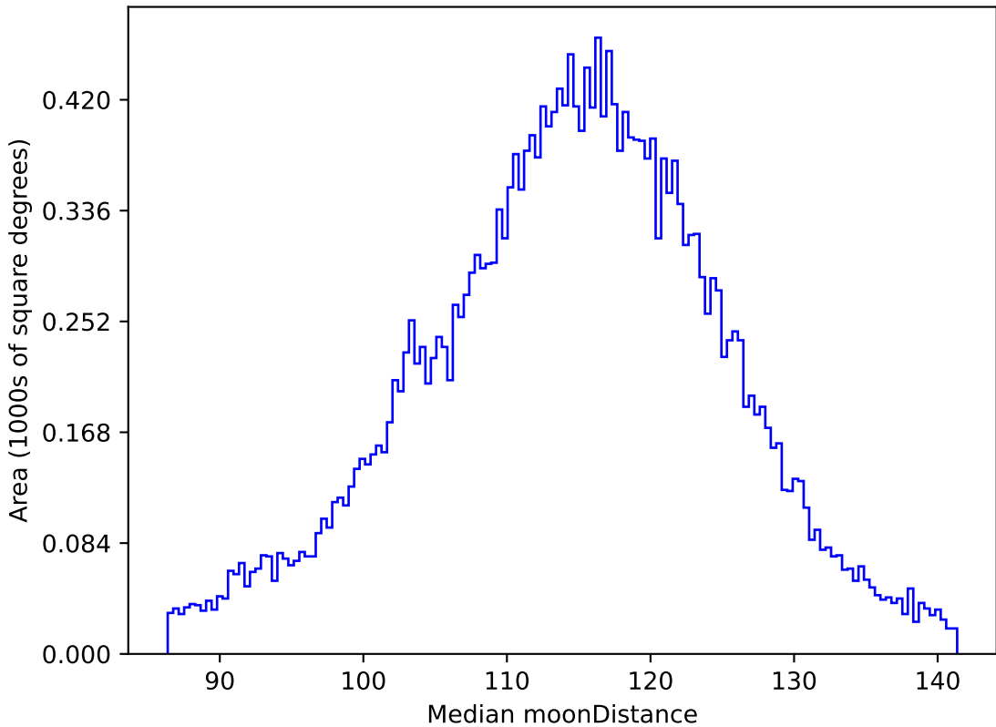
mw_roll_all_v3.3_10yrs All sky g band: Median moonDistance
