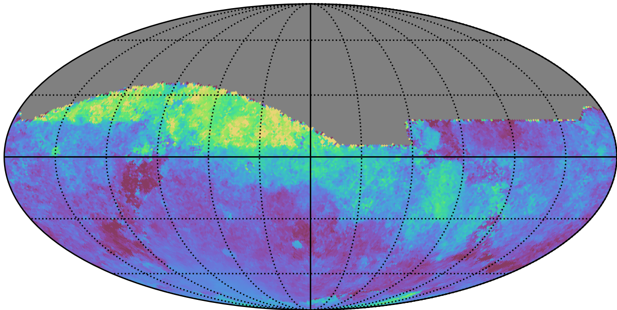
mw_roll_all_v3.3_10yrs All sky all bands: Median moonDistance
