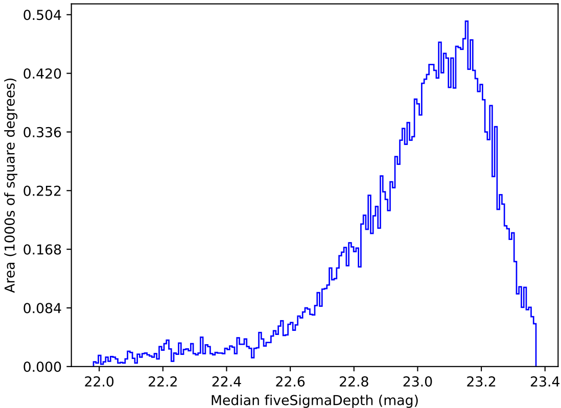
mw_roll_all_v3.3_10yrs Yr 1 z band: Median fiveSigmaDepth
