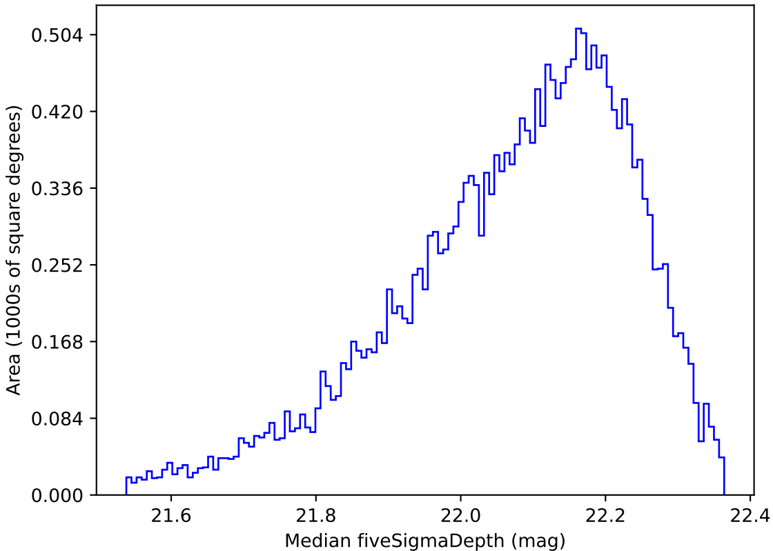
mw_roll_all_v3.3_10yrs Yr 1 y band: Median fiveSigmaDepth
