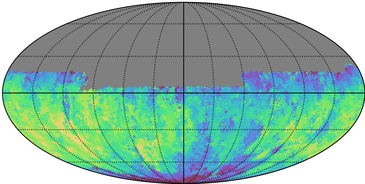
mw_roll_all_v3.3_10yrs Yr 1 u band: Median fiveSigmaDepth
