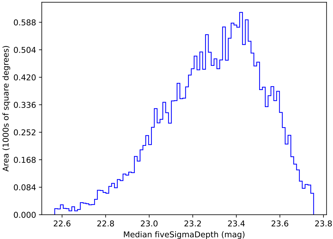
mw_roll_all_v3.3_10yrs Yr 1 u band: Median fiveSigmaDepth
