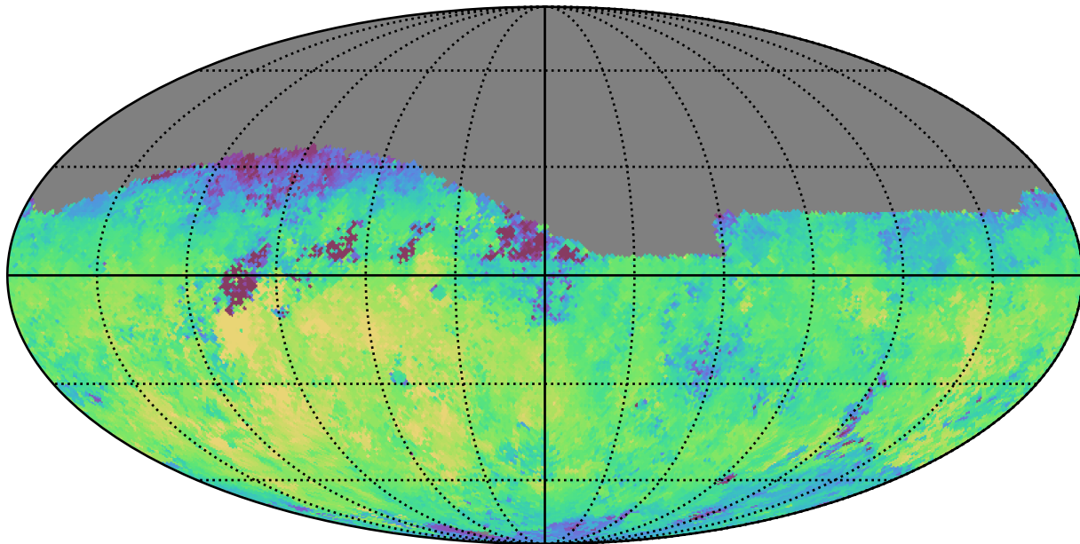
mw_roll_all_v3.3_10yrs Yr 1 r band: Median fiveSigmaDepth
