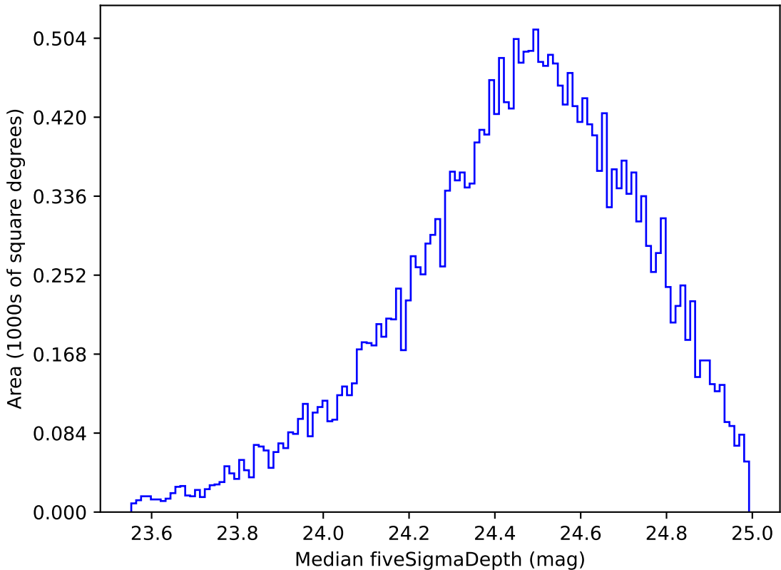
mw_roll_all_v3.3_10yrs Yr 1 g band: Median fiveSigmaDepth
