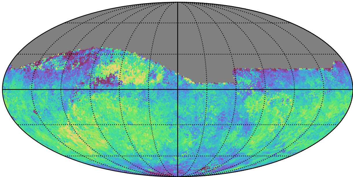
mw_roll_all_v3.3_10yrs Yr 1 all bands: Median fiveSigmaDepth
