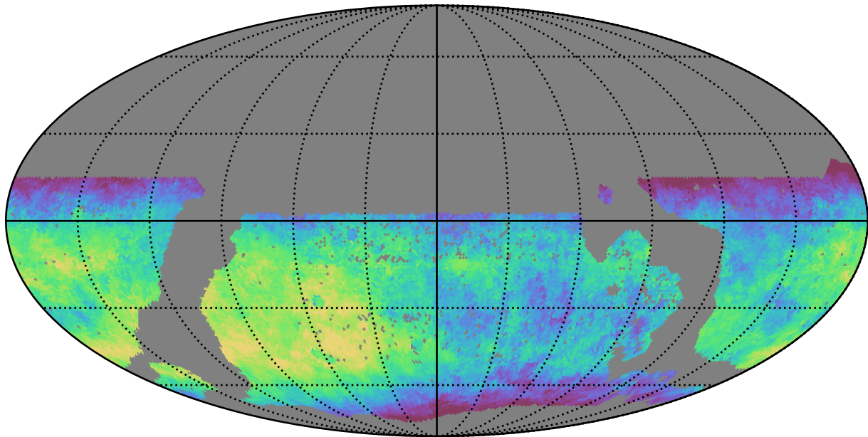
mw_roll_all_v3.3_10yrs WFD z band: Median fiveSigmaDepth
