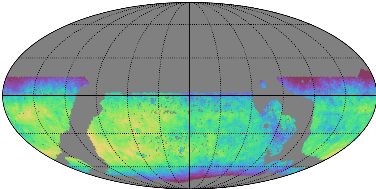
mw_roll_all_v3.3_10yrs WFD y band: Median fiveSigmaDepth
