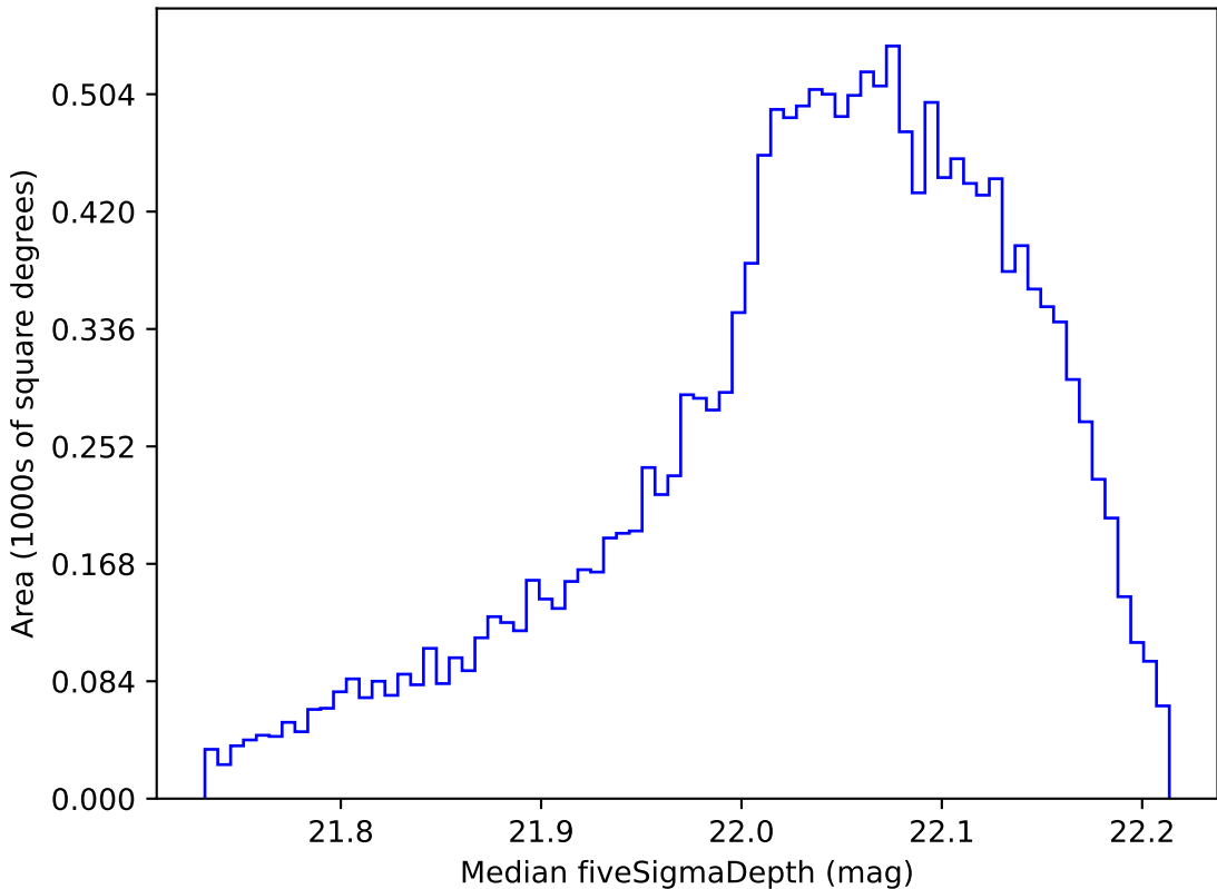
mw_roll_all_v3.3_10yrs WFD y band: Median fiveSigmaDepth
