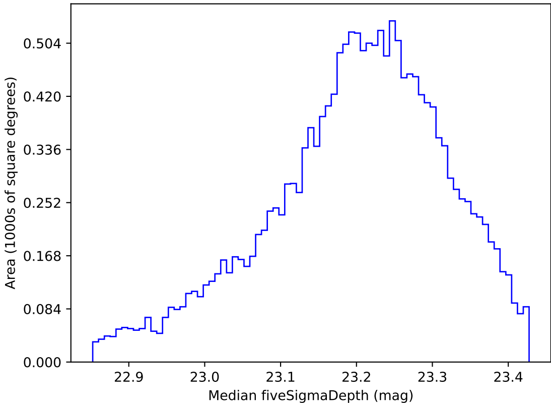
mw_roll_all_v3.3_10yrs WFD u band: Median fiveSigmaDepth
