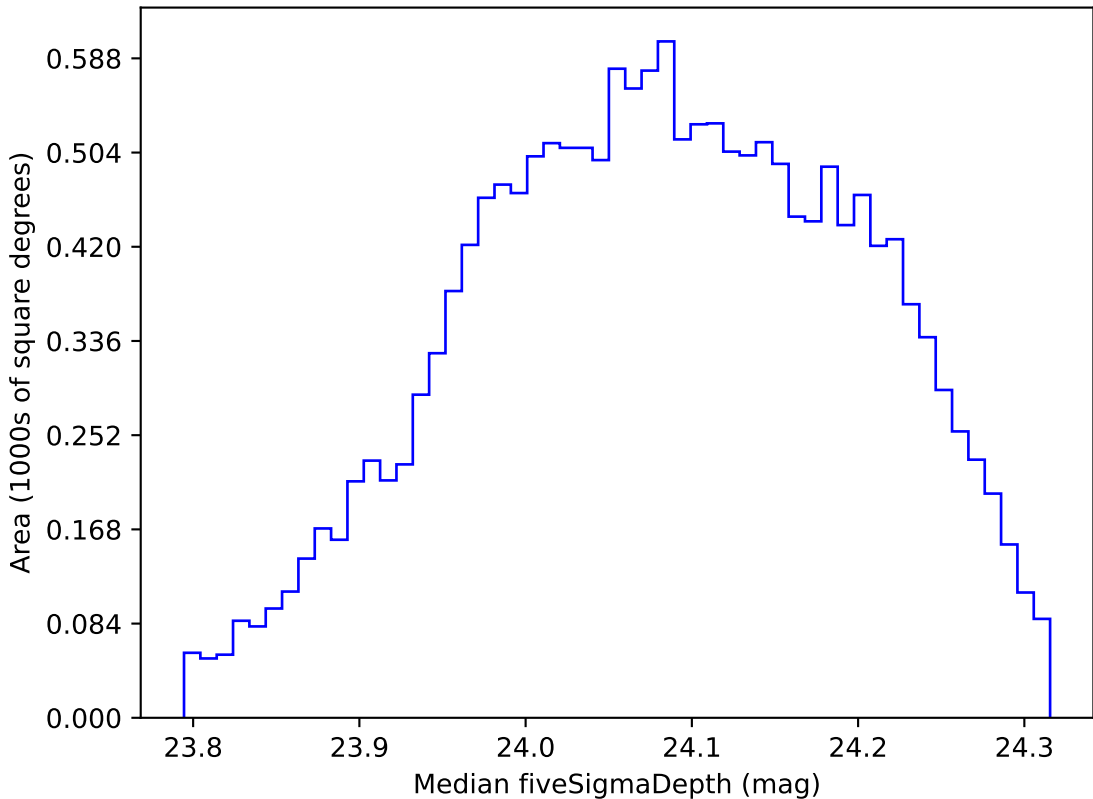
mw_roll_all_v3.3_10yrs WFD r band: Median fiveSigmaDepth
