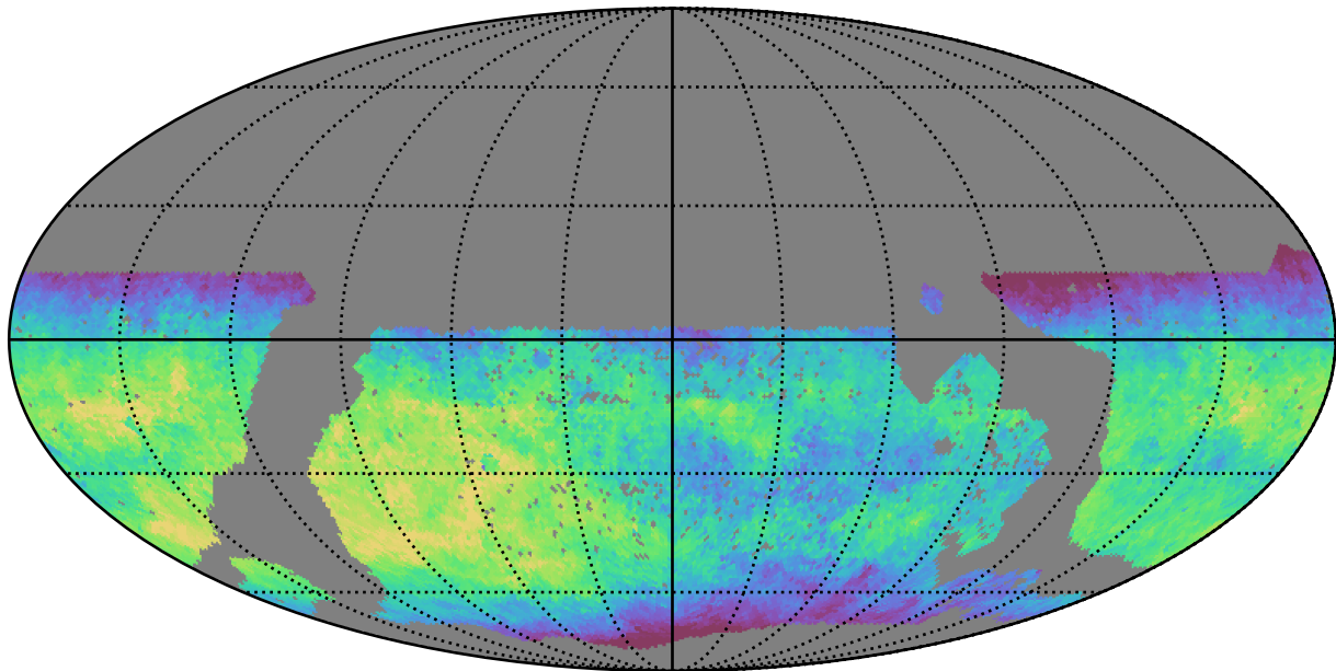
mw_roll_all_v3.3_10yrs WFD i band: Median fiveSigmaDepth
