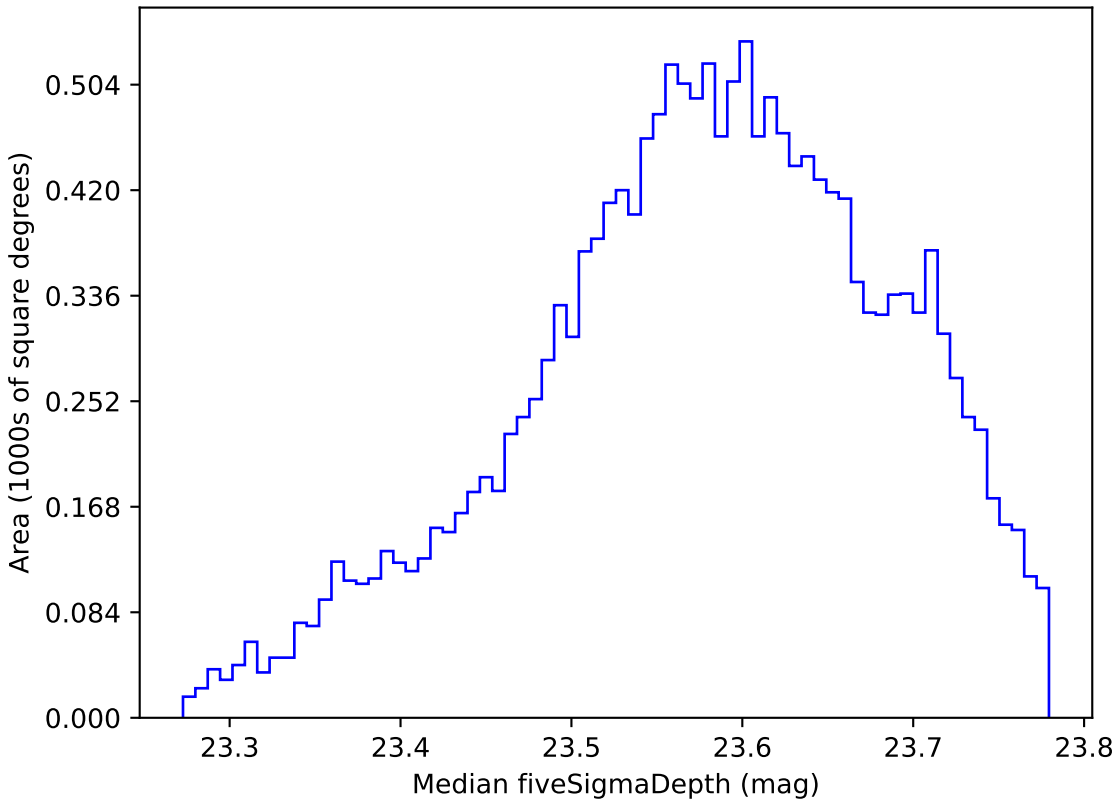
mw_roll_all_v3.3_10yrs WFD i band: Median fiveSigmaDepth
