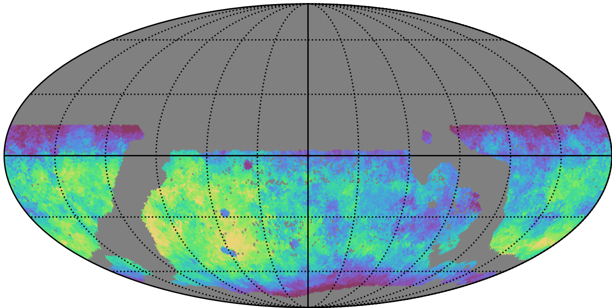
mw_roll_all_v3.3_10yrs WFD g band: Median fiveSigmaDepth
