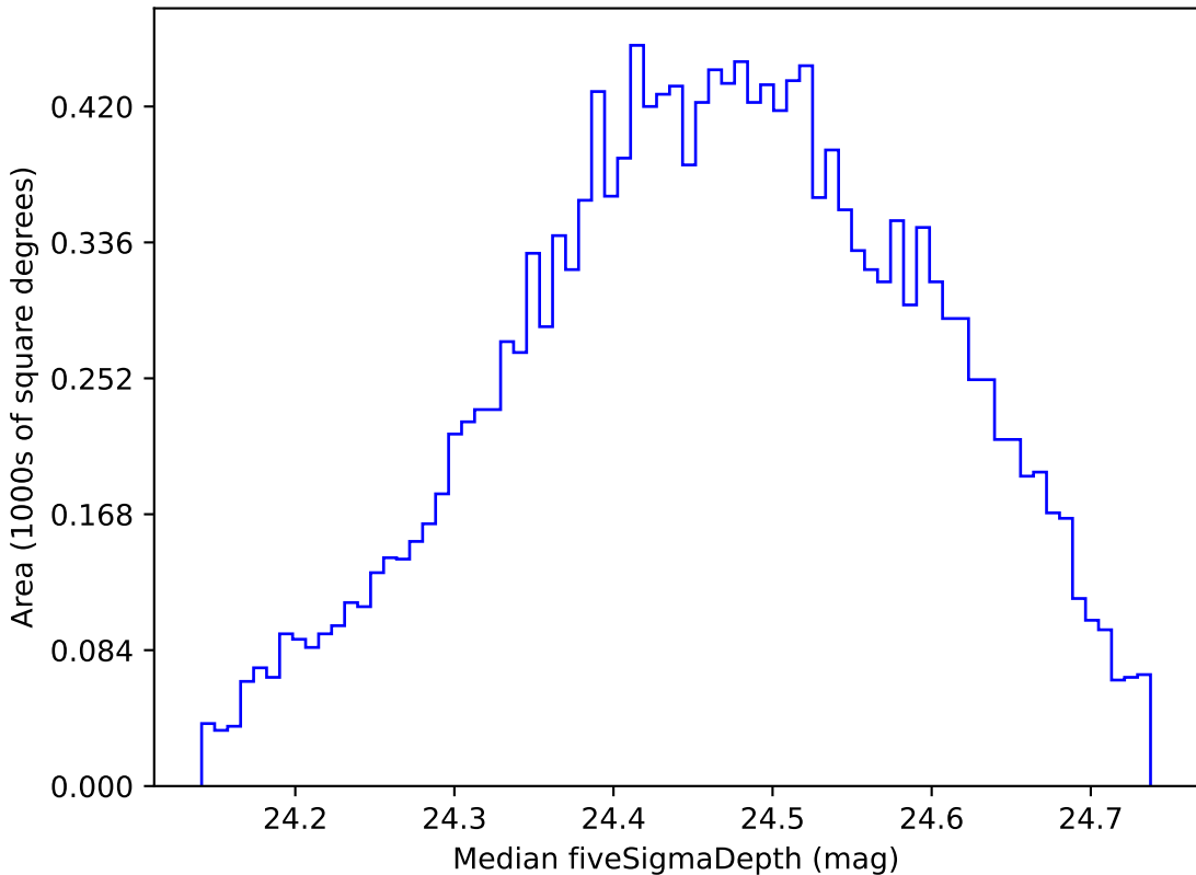
mw_roll_all_v3.3_10yrs WFD g band: Median fiveSigmaDepth
