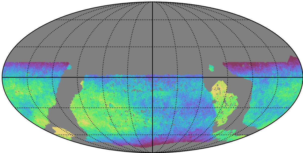
mw_roll_all_v3.3_10yrs WFD all bands: Median fiveSigmaDepth
