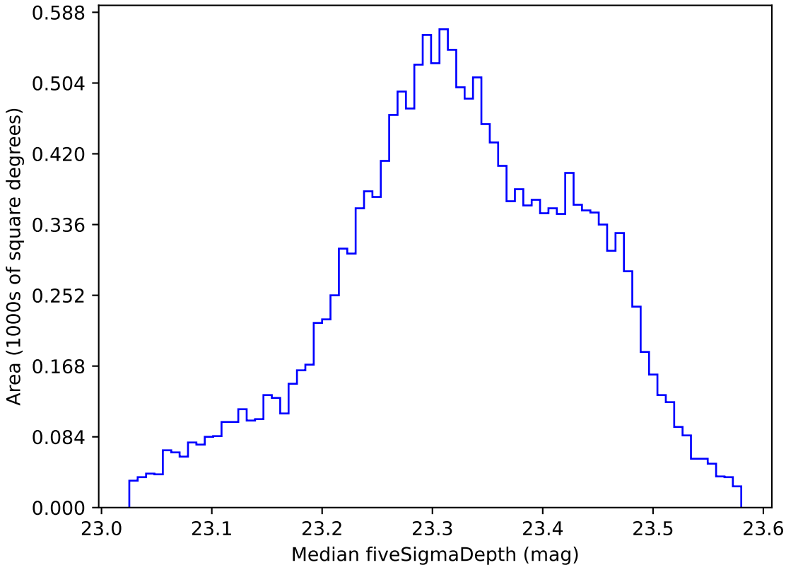
mw_roll_all_v3.3_10yrs WFD all bands: Median fiveSigmaDepth
