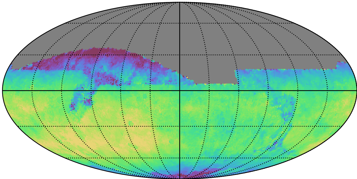
mw_roll_all_v3.3_10yrs All sky z band: Median fiveSigmaDepth
