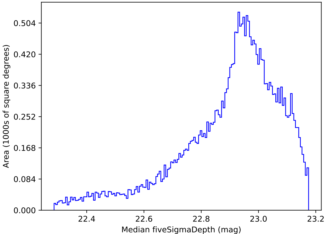
mw_roll_all_v3.3_10yrs All sky z band: Median fiveSigmaDepth
