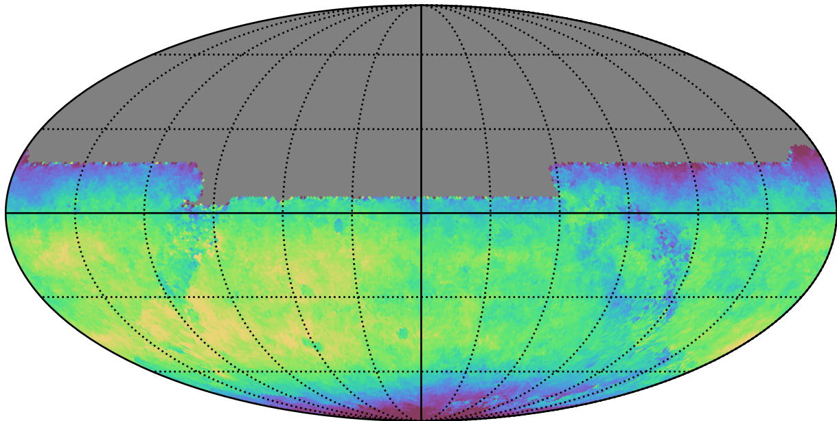
mw_roll_all_v3.3_10yrs All sky y band: Median fiveSigmaDepth
