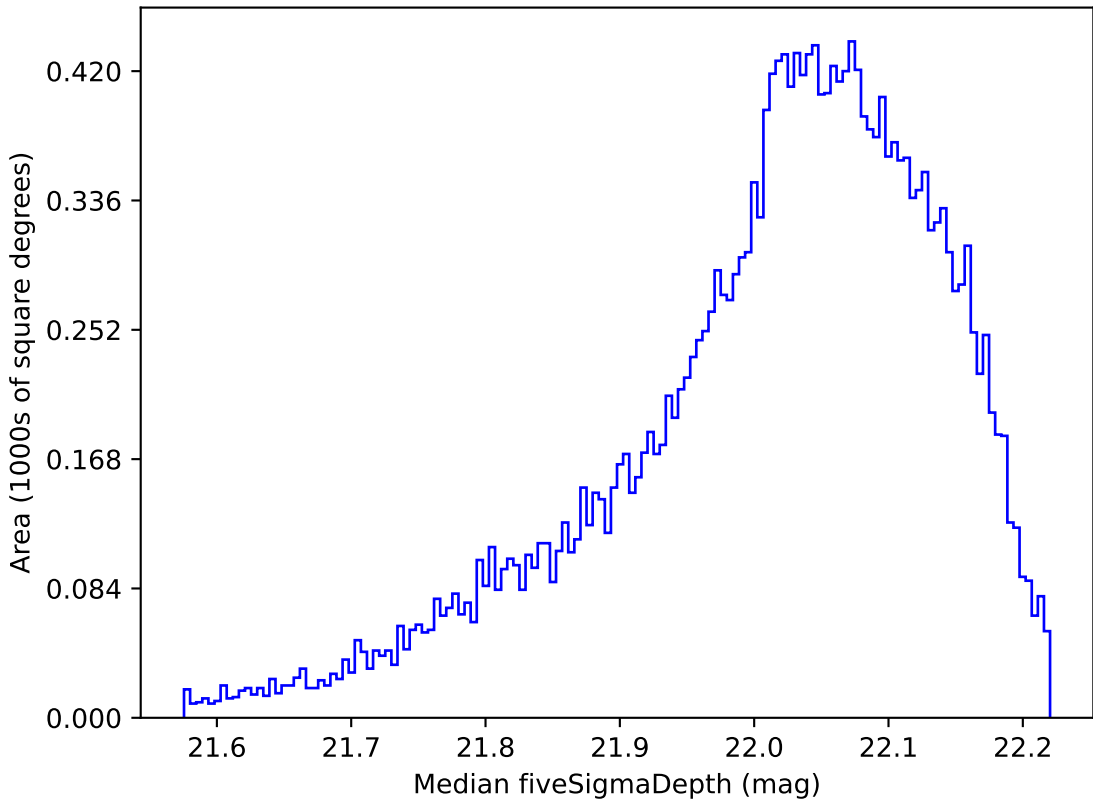
mw_roll_all_v3.3_10yrs All sky y band: Median fiveSigmaDepth
