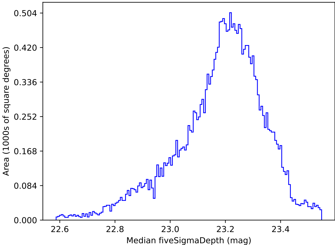
mw_roll_all_v3.3_10yrs All sky u band: Median fiveSigmaDepth
