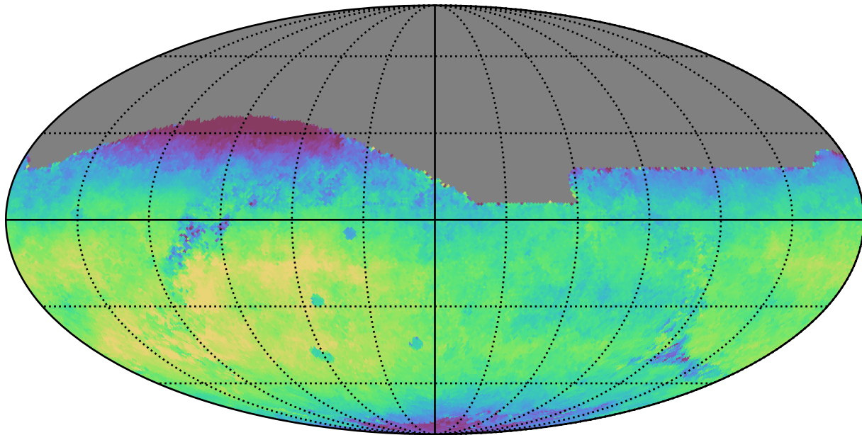
mw_roll_all_v3.3_10yrs All sky r band: Median fiveSigmaDepth
