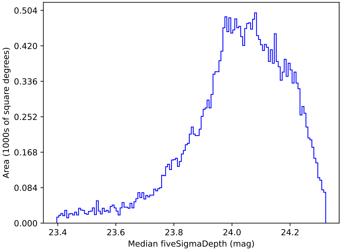
mw_roll_all_v3.3_10yrs All sky r band: Median fiveSigmaDepth
