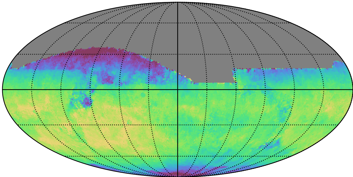
mw_roll_all_v3.3_10yrs All sky i band: Median fiveSigmaDepth
