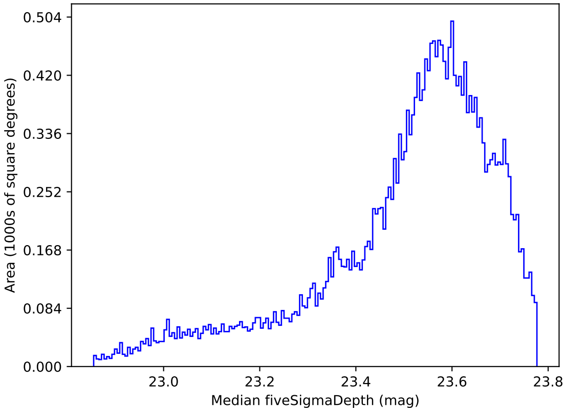
mw_roll_all_v3.3_10yrs All sky i band: Median fiveSigmaDepth
