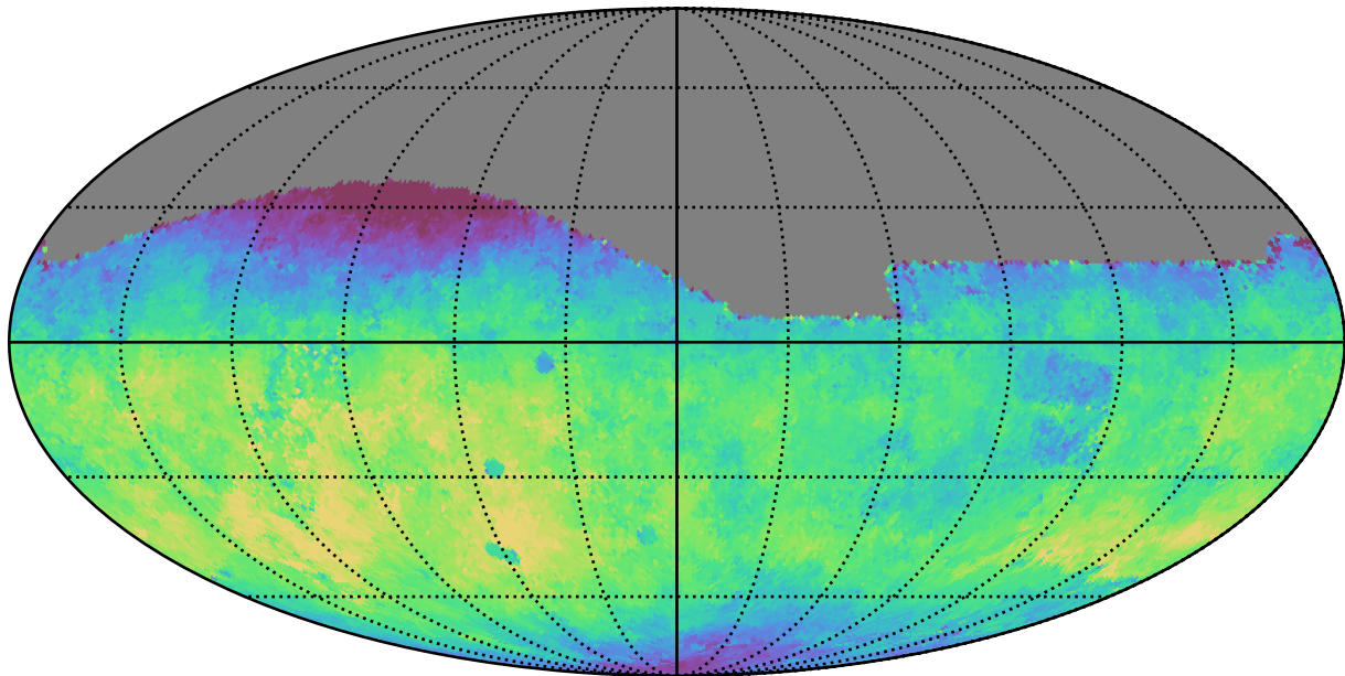
mw_roll_all_v3.3_10yrs All sky g band: Median fiveSigmaDepth
