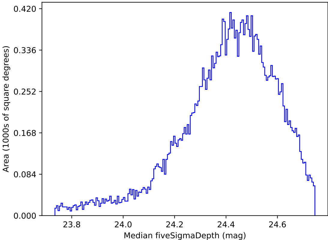
mw_roll_all_v3.3_10yrs All sky g band: Median fiveSigmaDepth
