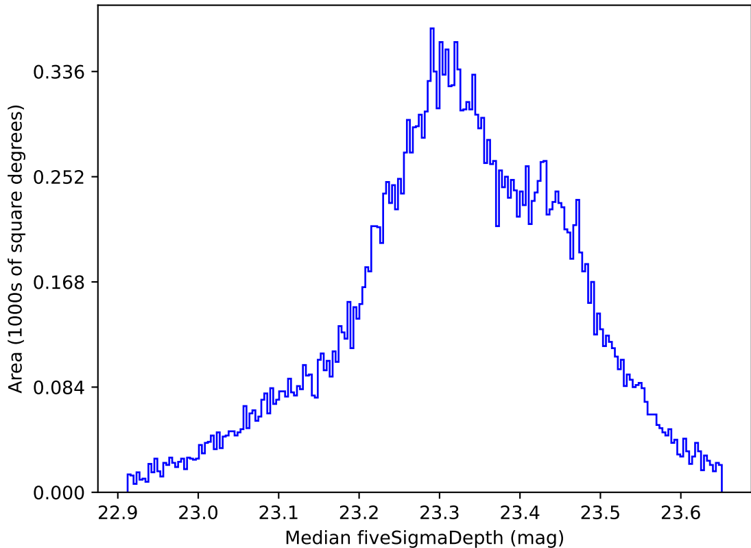
mw_roll_all_v3.3_10yrs All sky all bands: Median fiveSigmaDepth
