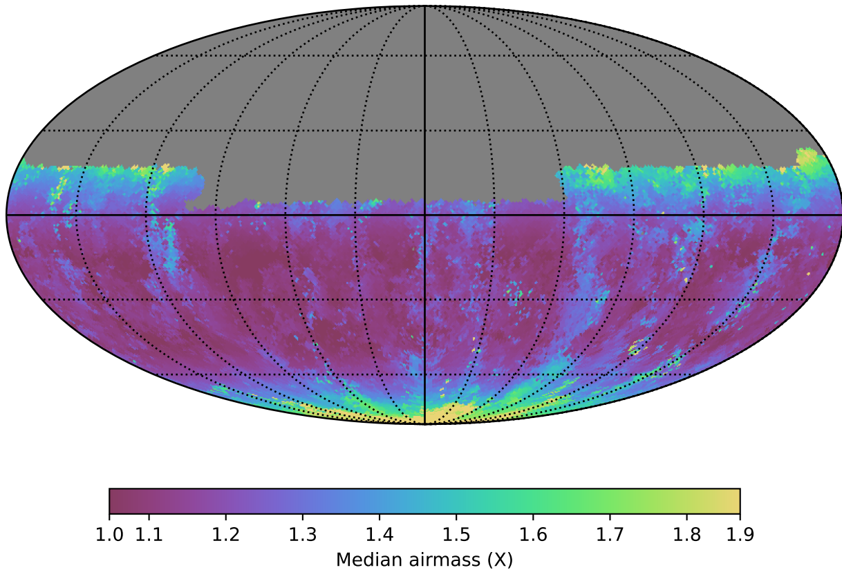
mw_roll_all_v3.3_10yrs Yr 1 u band: Median airmass
