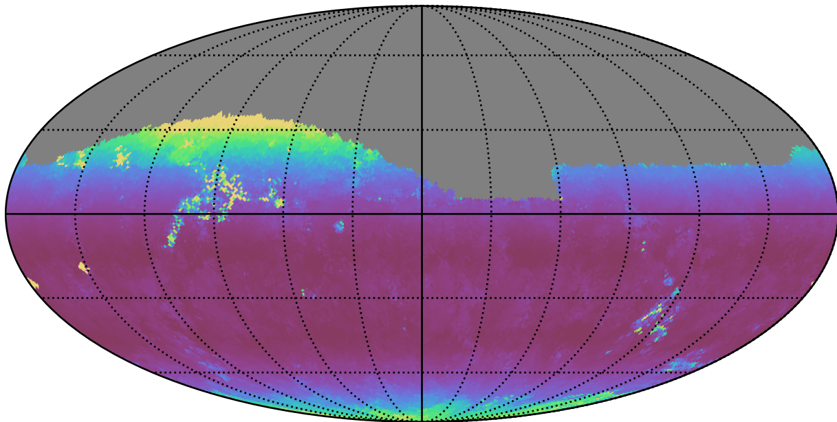
mw_roll_all_v3.3_10yrs Yr 1 i band: Median airmass
