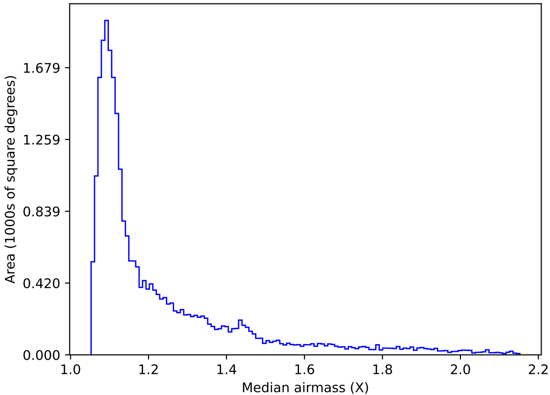
mw_roll_all_v3.3_10yrs Yr 1 i band: Median airmass
