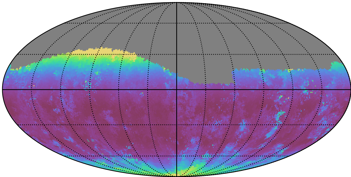
mw_roll_all_v3.3_10yrs Yr 1 g band: Median airmass
