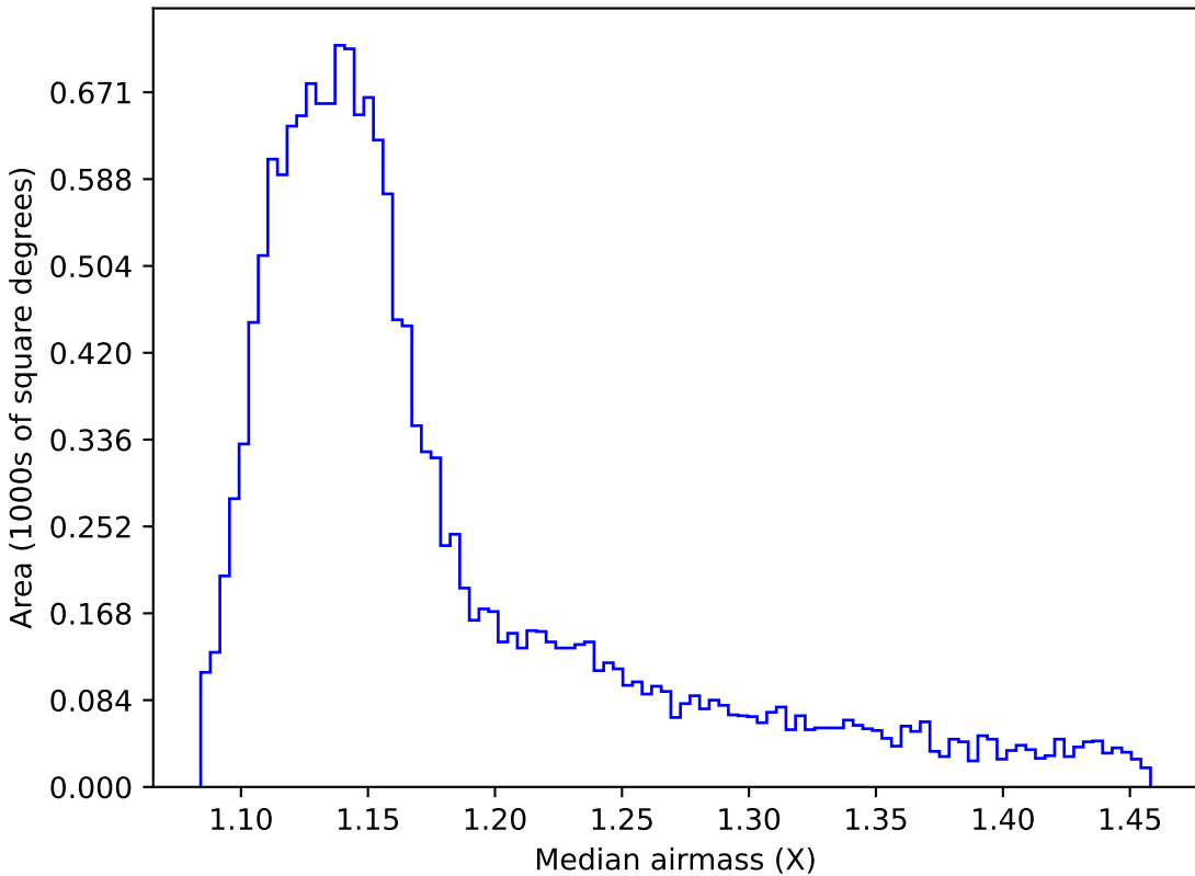
mw_roll_all_v3.3_10yrs WFD z band: Median airmass
