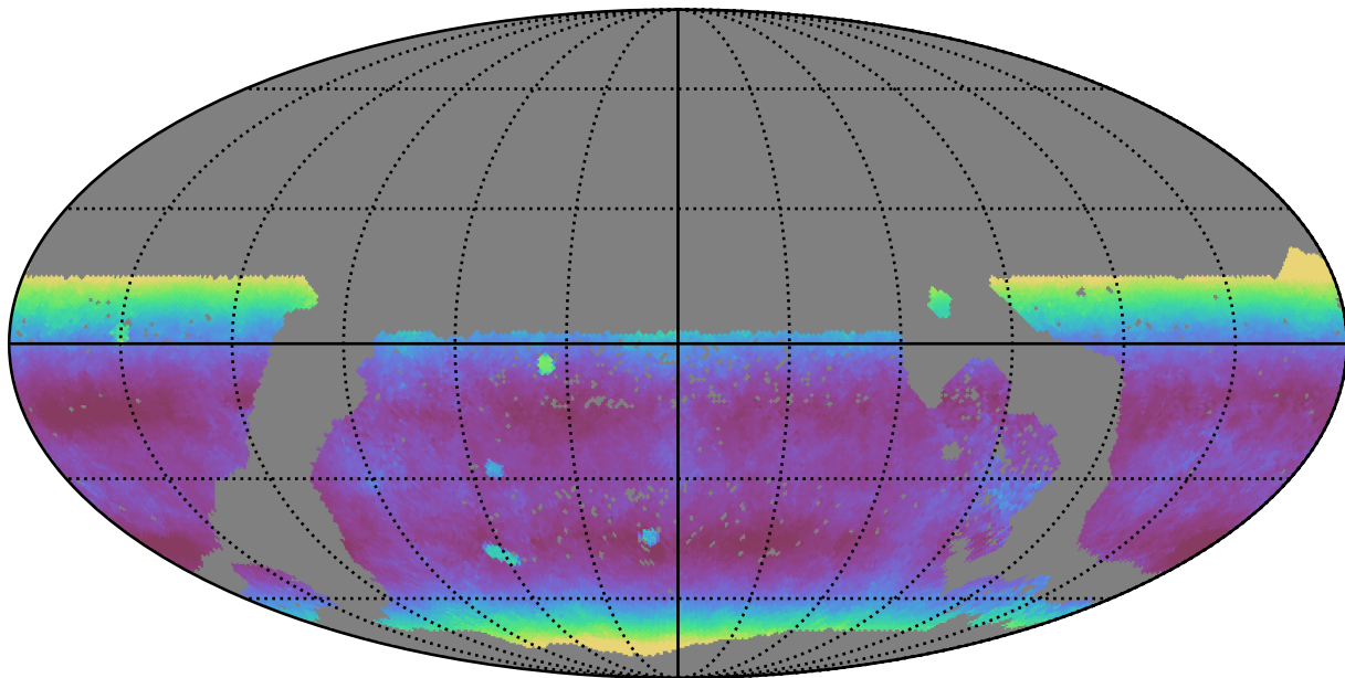
mw_roll_all_v3.3_10yrs WFD y band: Median airmass
