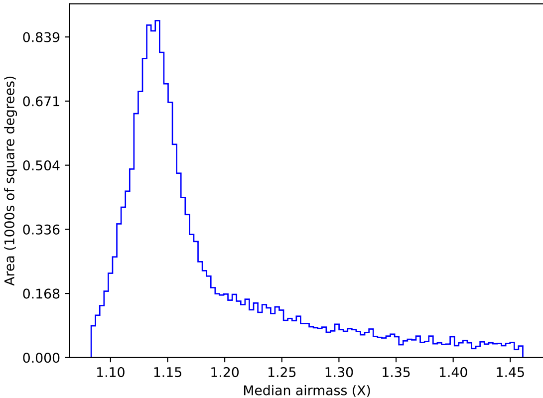
mw_roll_all_v3.3_10yrs WFD y band: Median airmass
