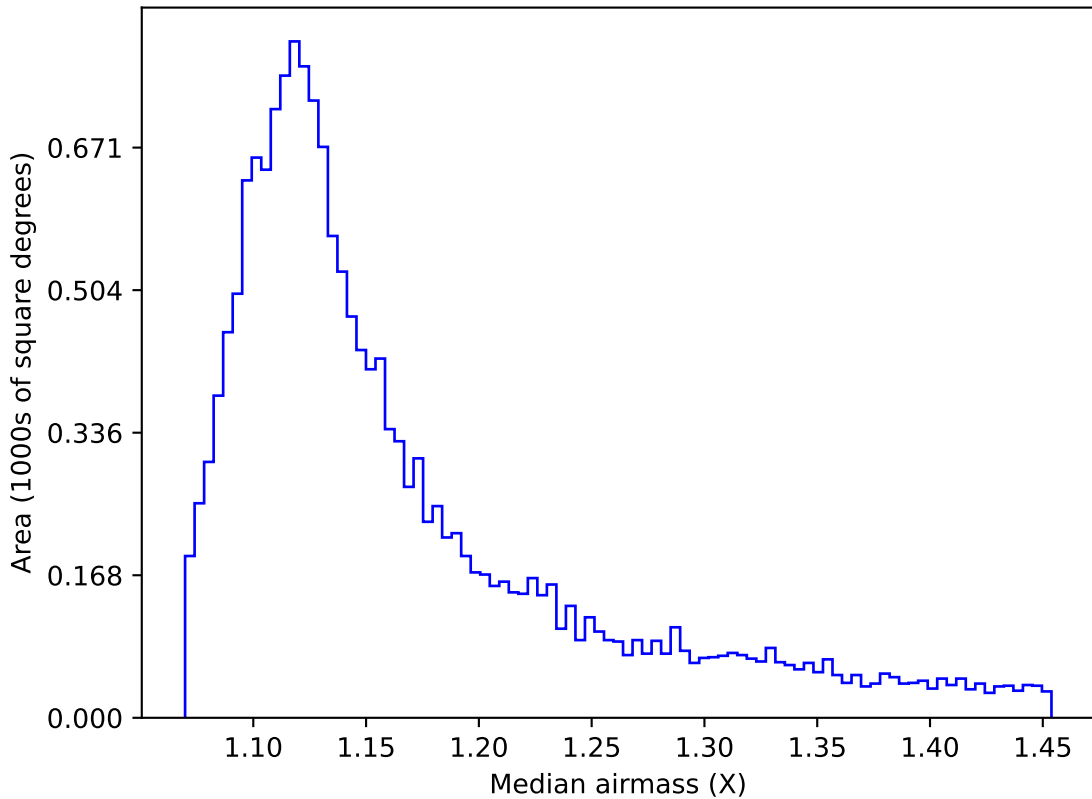
mw_roll_all_v3.3_10yrs WFD u band: Median airmass
