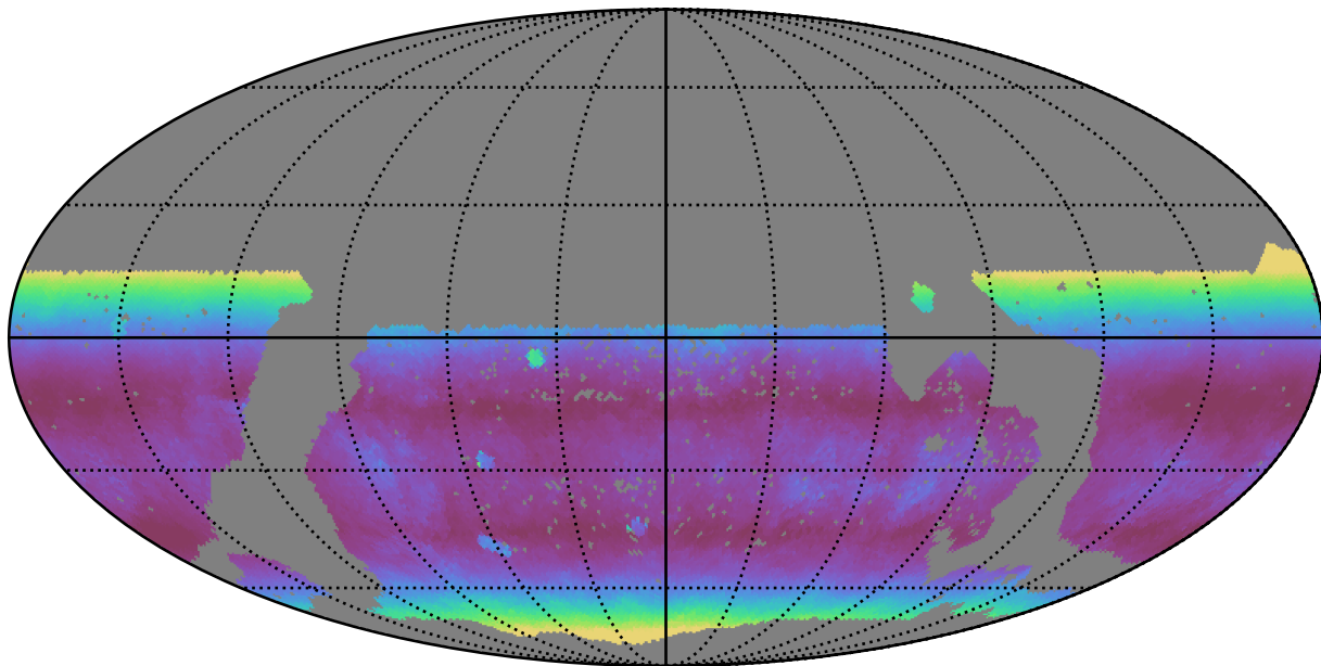
mw_roll_all_v3.3_10yrs WFD r band: Median airmass
