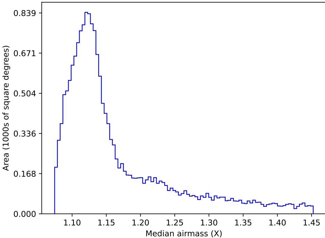
mw_roll_all_v3.3_10yrs WFD r band: Median airmass
