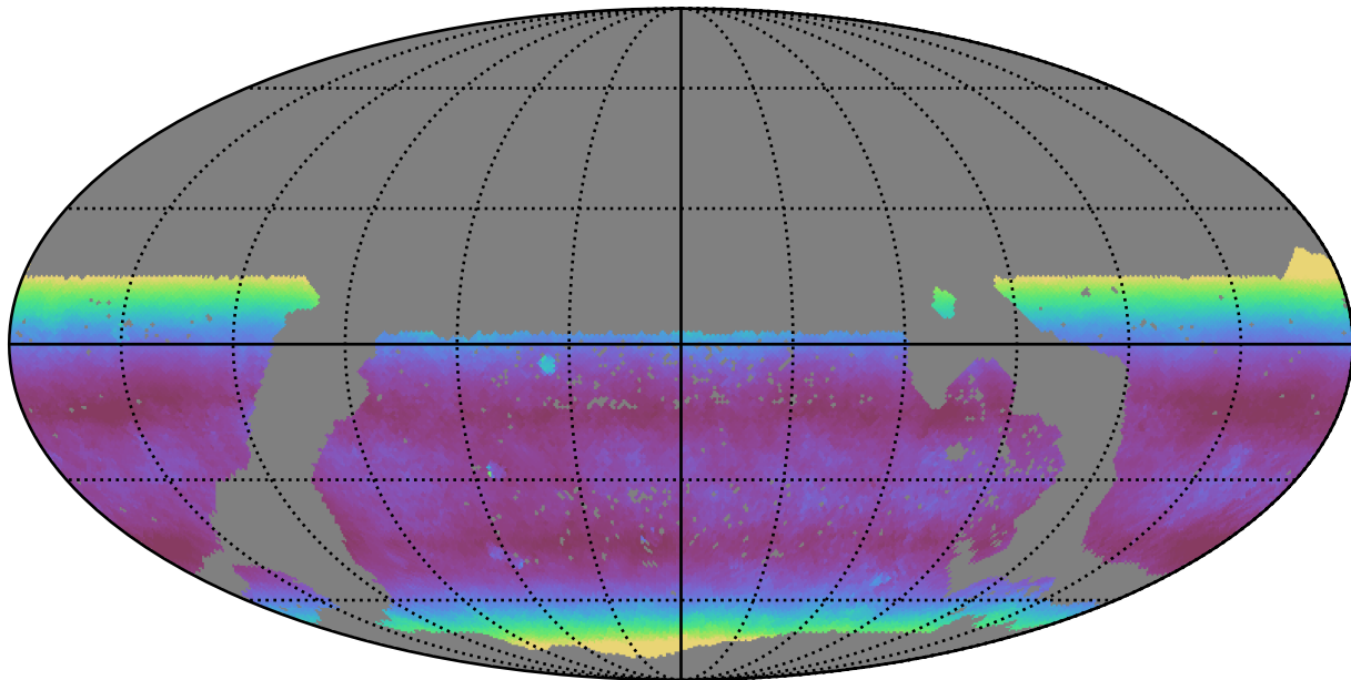
mw_roll_all_v3.3_10yrs WFD i band: Median airmass
