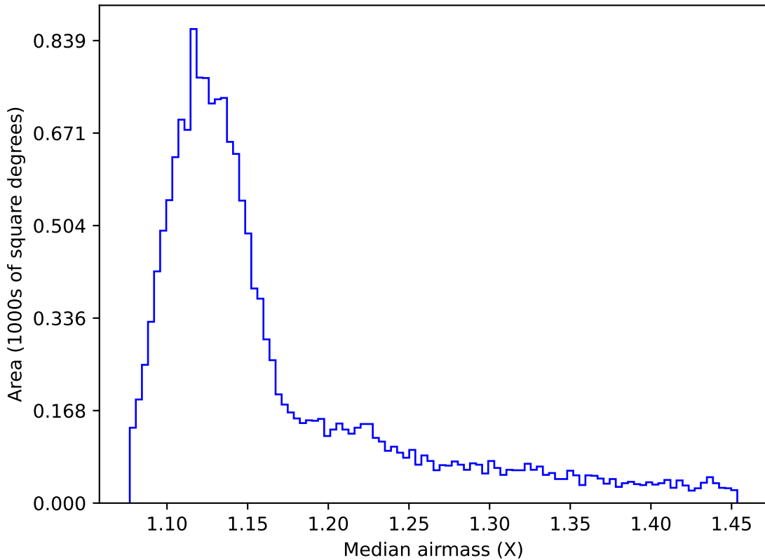
mw_roll_all_v3.3_10yrs WFD i band: Median airmass
