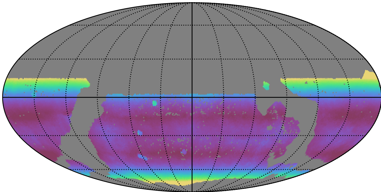
mw_roll_all_v3.3_10yrs WFD all bands: Median airmass
