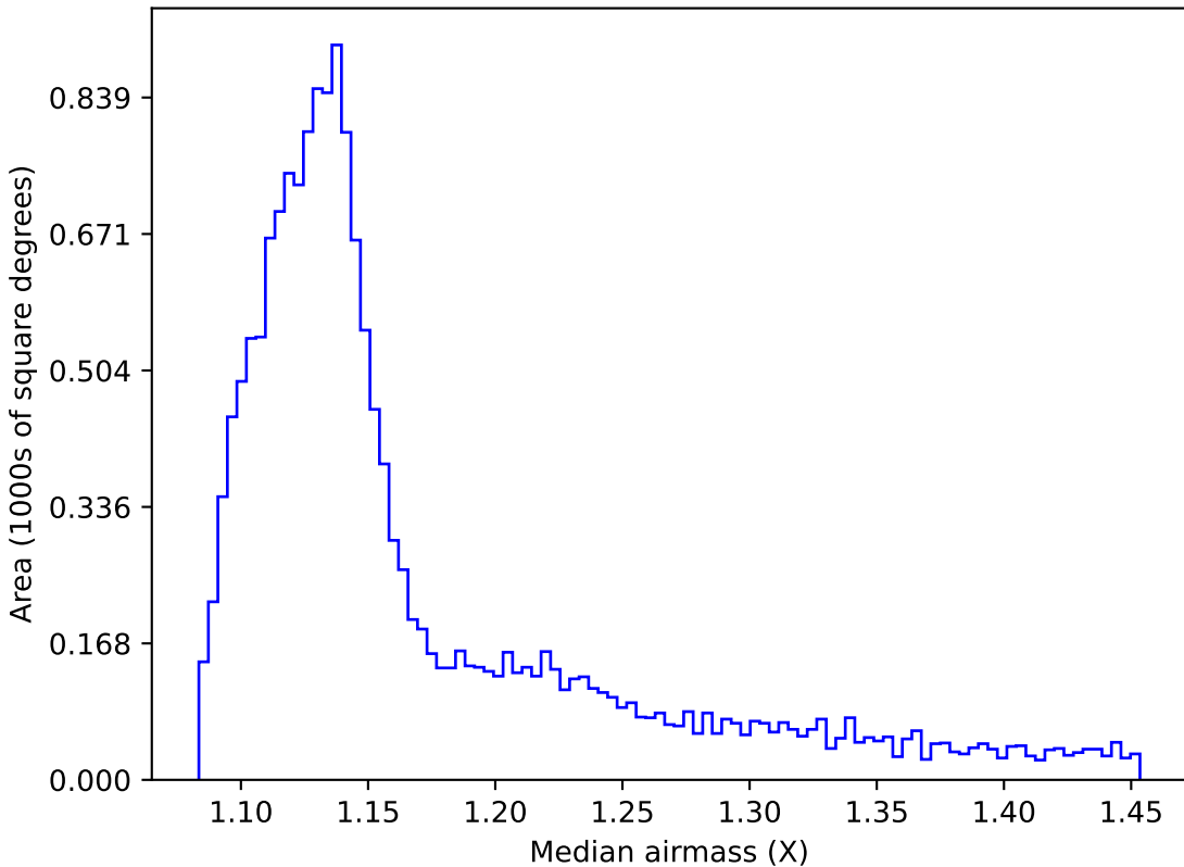
mw_roll_all_v3.3_10yrs WFD all bands: Median airmass
